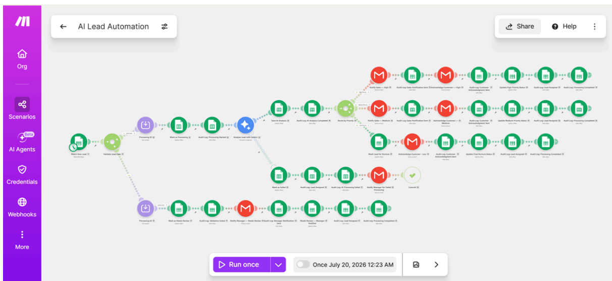
Figure 1. Main lead-processing workflow in Make.com
