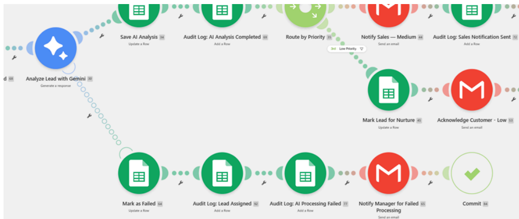
Figure 11. Gemini failure-handling route
