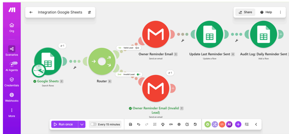
Figure 2. Follow-up reminder scenario
